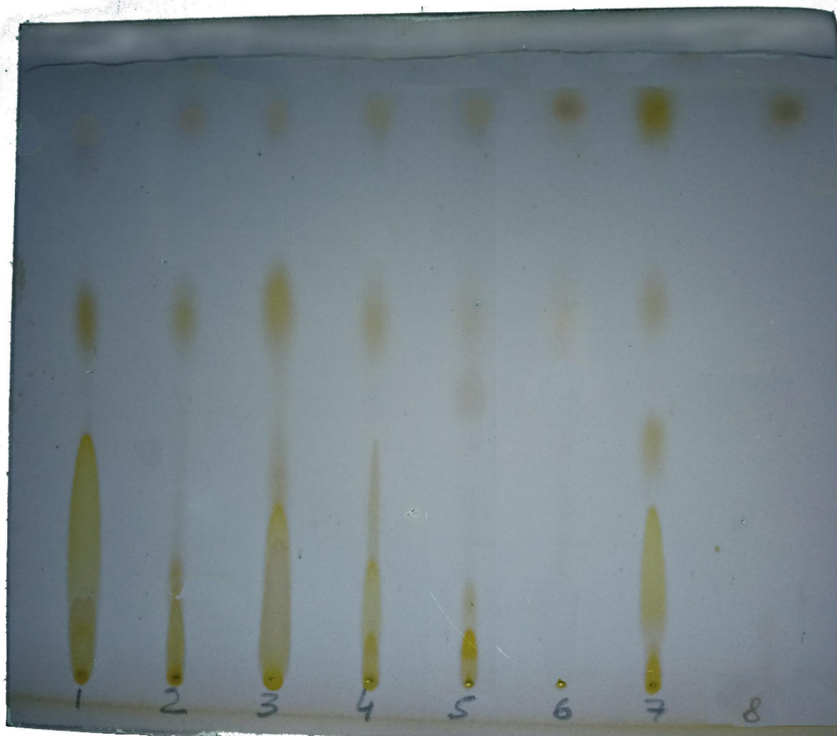
Supplementary Fig. S1 - Thin-layer chromatogram of lipophilic fractions of fungi and squalene. Numbers indicate the tracks of lipophilic extracts: 1 - Mucidula mucida , 2 - Lycoperdon pyriforme , 3 - Laetiporus sulphureus , 4 - Tyromyces chioneus , 5 - Sarcoscypha coccinea , 6 - fractions 1-4 of the lipophilic extract of Sarcoscypha coccinea (Fig. 1), 7 - Amaranthus caudatus , 8 - squalene from Sigma-Aldrich.
